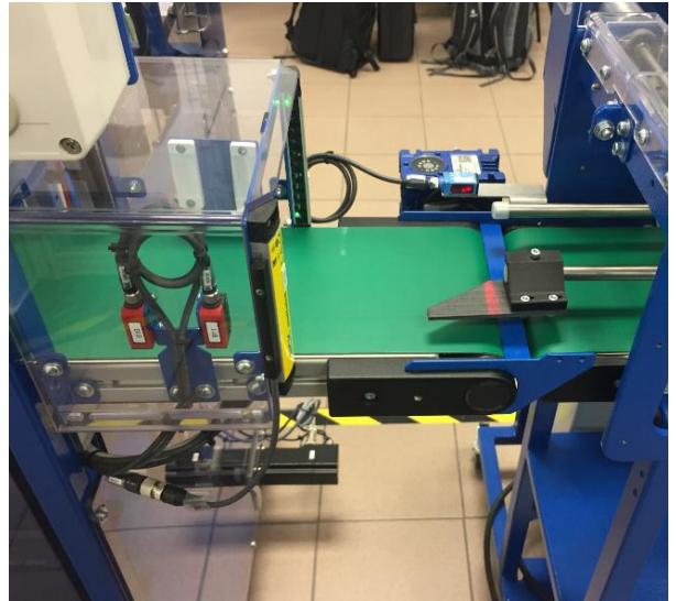
Light curtain at the conveyor entrance
