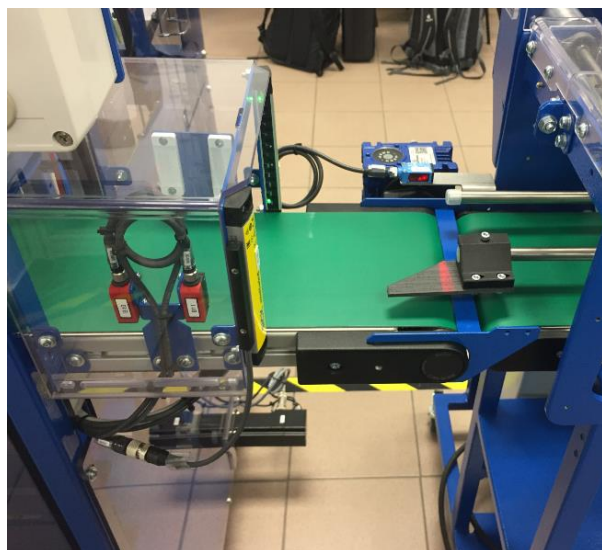
Light curtain at the conveyor entrance
